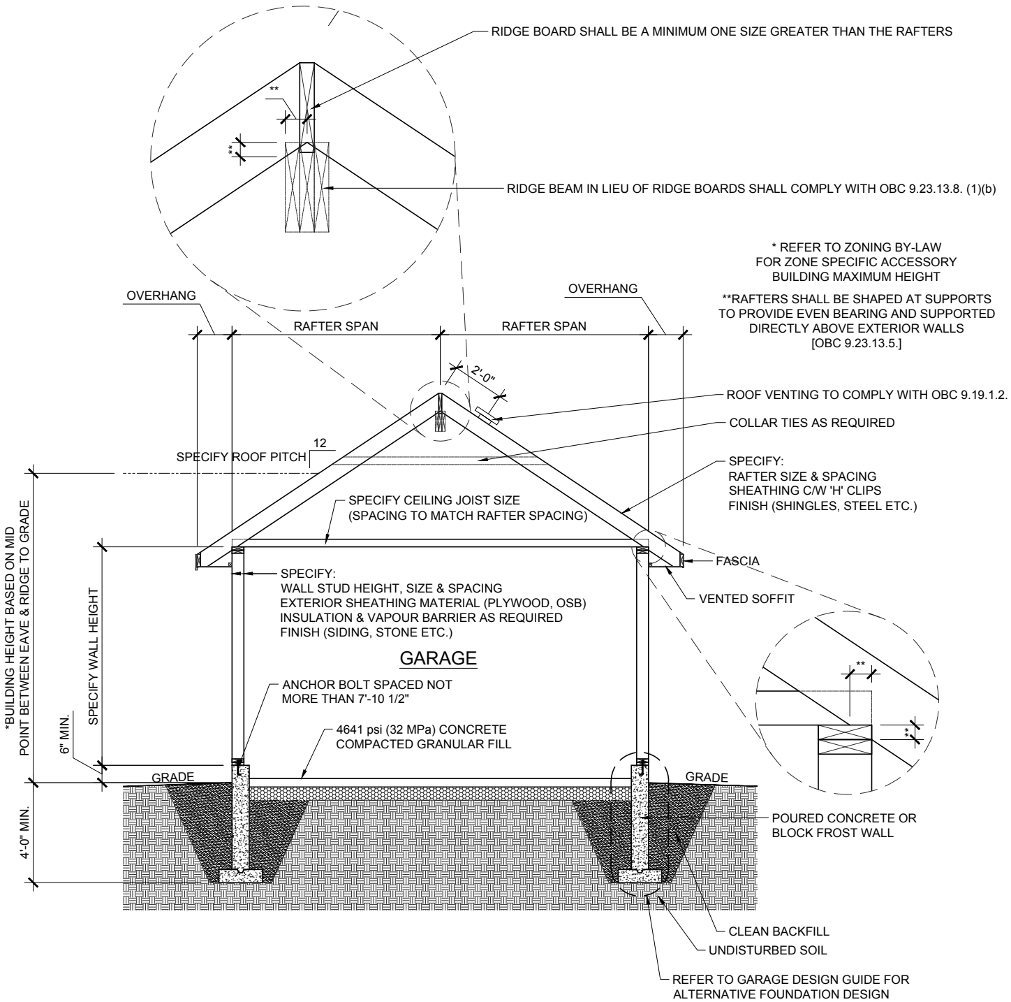
SAMPLE GARAGE/ACCESSORY CROSS SECTION
