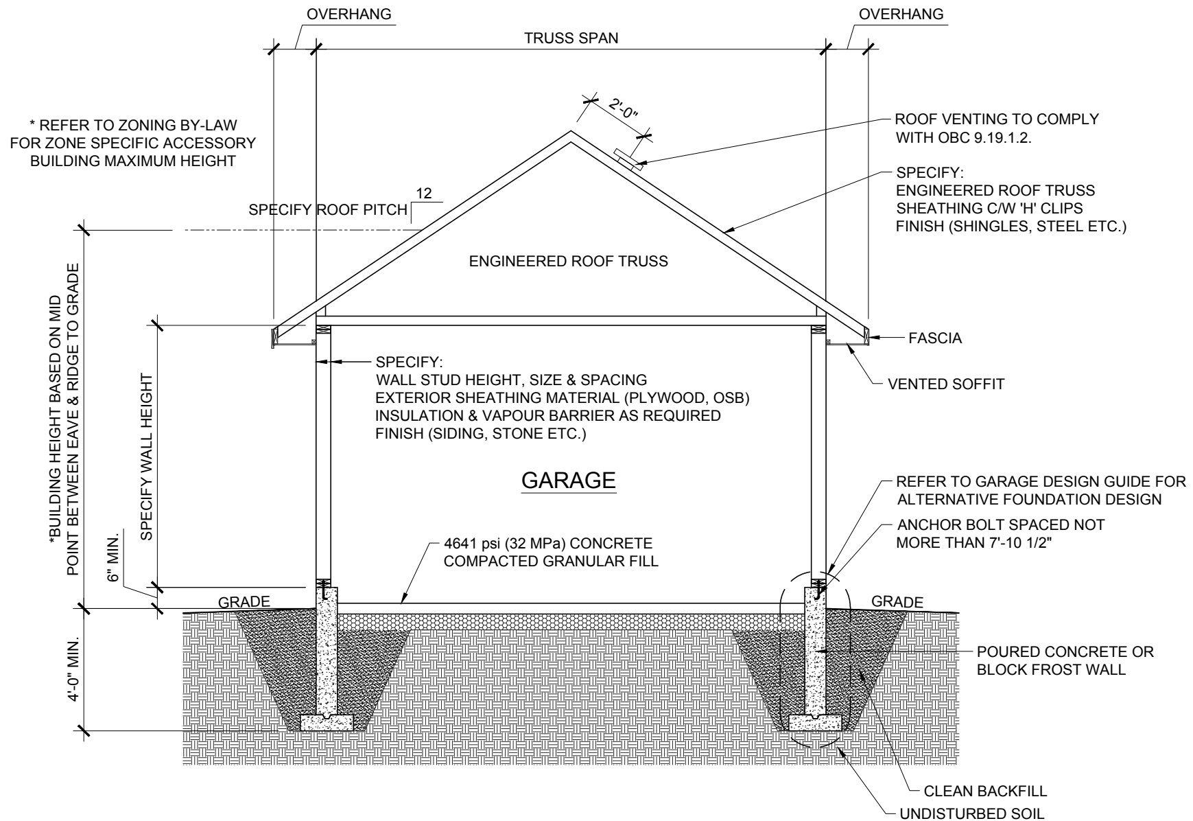
SAMPLE GARAGE/ACCESSORY CROSS SECTION
