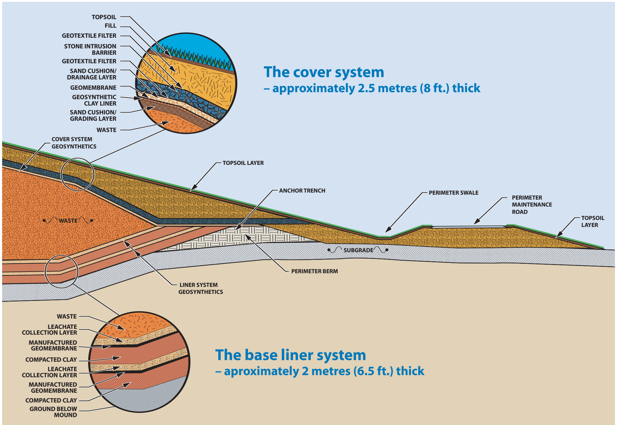
Cross-section of conceptual design
