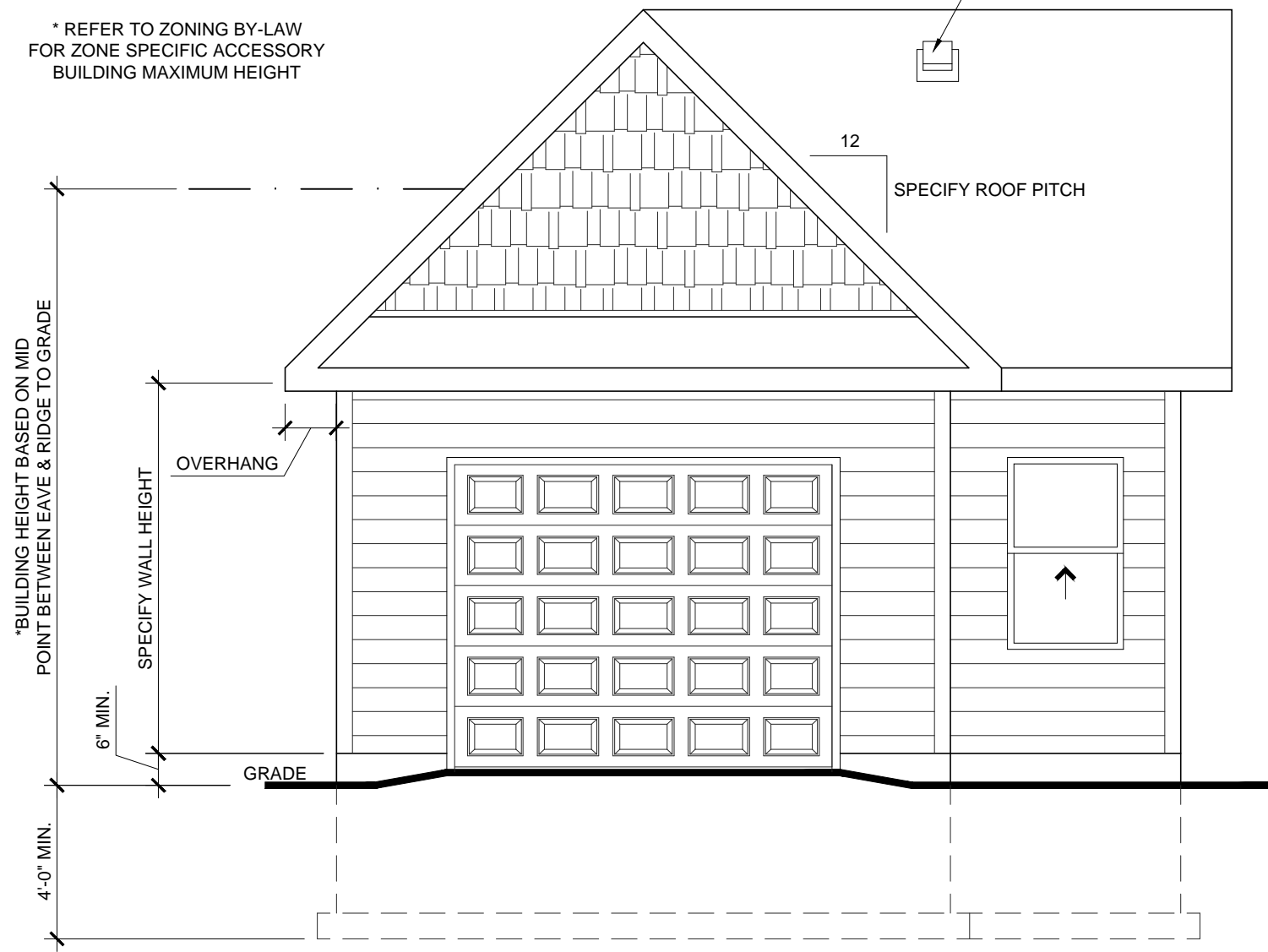
SAMPLE GARAGE/ACCESSORY ELEVATION
